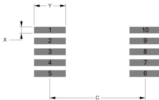
Figure 12.2 MSOP-10 Footprint.
