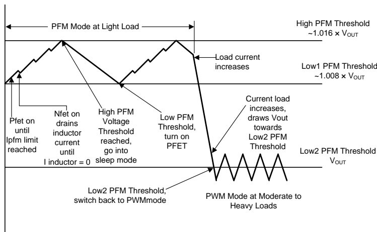
Figure 20. PWM/PFM Modulation
